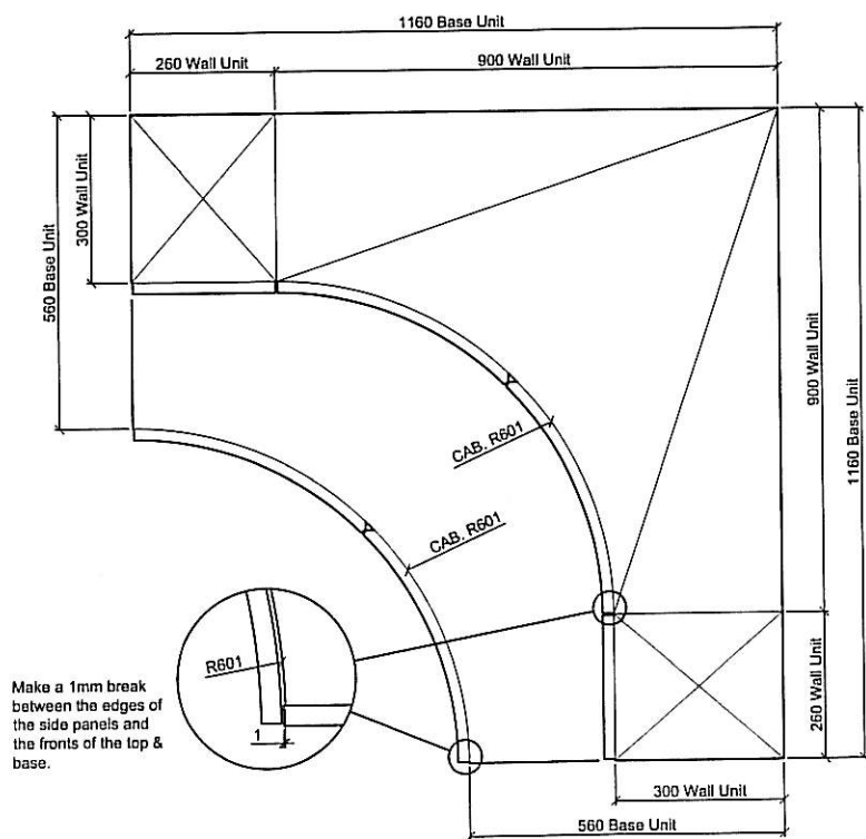
Concave Application 4 uses four Large concave doors & two 255mm wide doors
